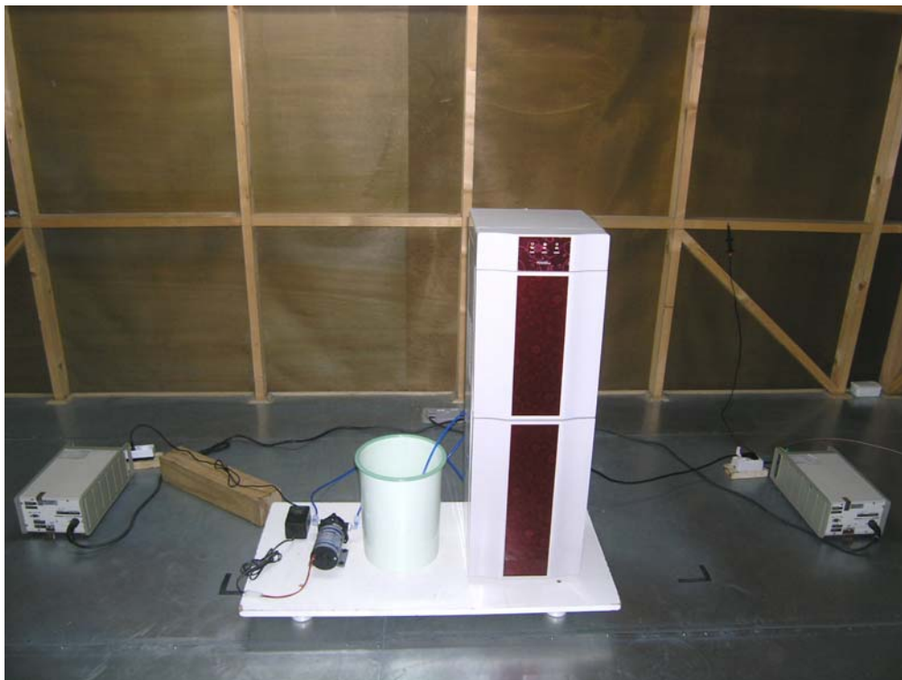
Photograph of test setup: Conducted emissions
