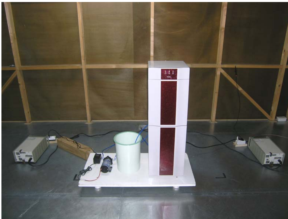
Photograph of test setup: Discontinuous Disturbance Emissions
